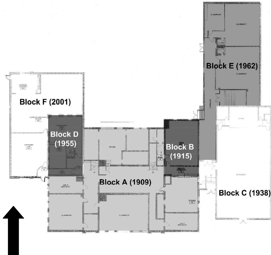
Figure 7. Hall School Blocks A-F (Basement Floor Plan).
